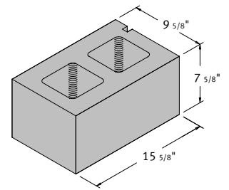
10 x 8 x 16 Semi Solid Pier
