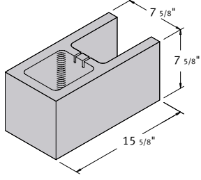
8 x 8 x 16 A Shaped Block
