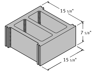
16 x 8 x 16 Hollow Stretcher
