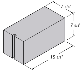
8 x 8 x 16 Solid Corner Sash
