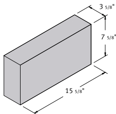
4 x 8 x 16 Solid Pier
