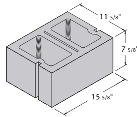
12 x 8 x 16 Hollow Double Sash
