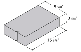
10 x 4 x 16 Solid Corner Sash
