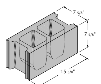
8 x 8 x 16 Hollow Cap
