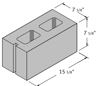
8 x 8 x 16 Semi Solid Corner Sash
