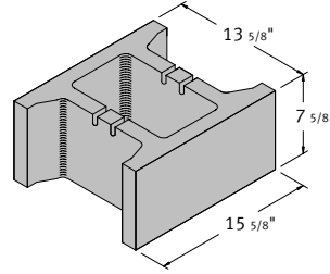
14 x 8 x 16 Open End
