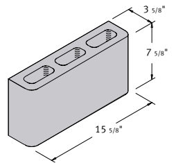
4 x 8 x 16 Hollow Single Bullnose Pier
