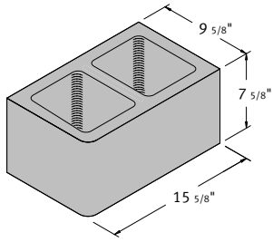
10 x 8 x 16 Hollow Single Bullnose Pier
