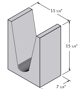
12 x 16 x 8 Bond Beam Lintel
