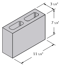
4 x 8 x 12 Hollow Pier
