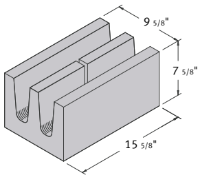
10 x 8 x 16 Solid-Bottom Bond Beam
