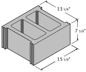
14 x 8 x 16 Hollow Stretcher
