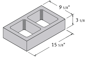
10 x 4 x 16 Hollow Pier
