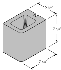
6 x 8 x 8 Hollow Single Bullnose Corner Sash
