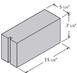
6 x 8 x 16 Solid Corner Sash
