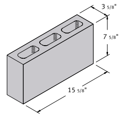
4 x 8 x 16 Hollow Pier
