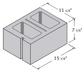
12 x 8 x 16 Hollow Corner Sash
