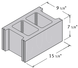
10 x 8 x 16 Hollow Stretcher
