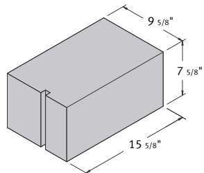
10 x 8 x 16 Solid Corner Sash
