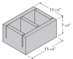
12 x 8 x 16 Knock-Out Bond Beam
