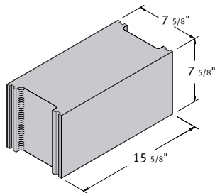
8 x 8 x 16 Solid Stretcher
