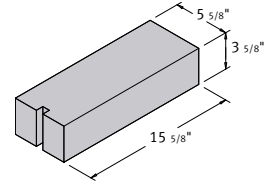
6 x 4 x 16 Solid Corner Sash
