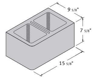
10 x 8 x 16 Hollow Single Bullnose Corner
