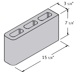
4 x 8 x 16 Hollow Double Bullnose Corner
