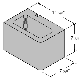
12 x 8 x 8 Hollow Single Bullnose Corner Sash
