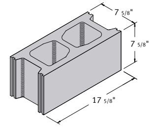
8 x 8 x 18 Hollow Stretcher
