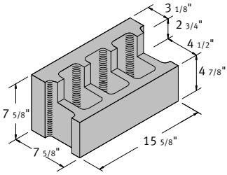
8 x 8 x 16 Hollow Header
