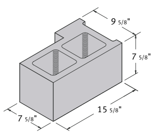
10 x 8 x 16 Hollow Return Corner
