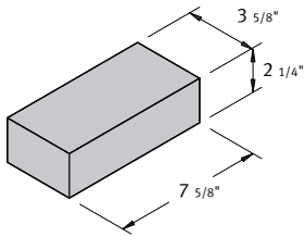
4 x 2 1/4 x 8 Concrete Brick
