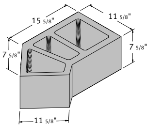
12 x 8 x 21 45 Degree Angle
