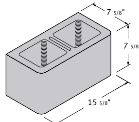
8 x 8 x 16 Hollow Single Bullnose Pier
