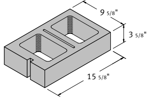
10 x 4 x 16 Hollow Corner Sash
