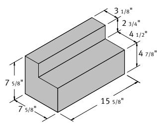
8 x 8 x 16 Solid Header Pier
