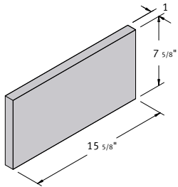
1 x 8 x 16 Solid Pier
