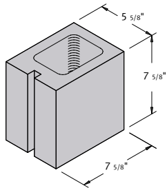
6 x 8 x 8 Hollow Corner Sash
