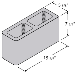
6 x 8 x 16 Hollow Double Bullnose Corner
