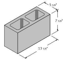
6 x 8 x 14 Hollow Pier
