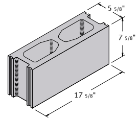
6 x 8 x 18 Hollow Stretcher
