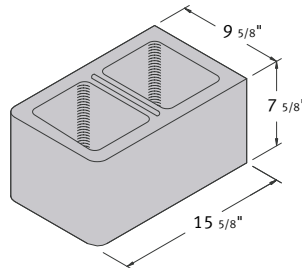
10 x 8 x 16 Hollow Double Bullnose Corner
