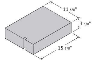
12 x 4 x 16 Solid Corner Sash
