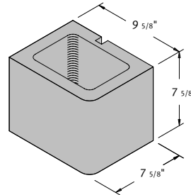
10 x 8 x 8 Hollow Single Bullnose Corner Sash
