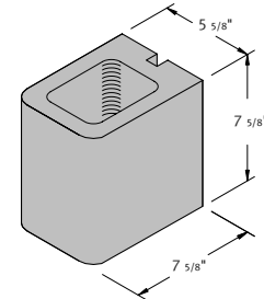
6 x 8 x 8 Hollow Double Bullnose Corner Sash
