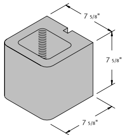
8 x 8 x 8 Hollow Double Bullnose Corner Sash
