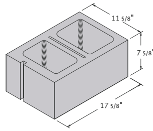
12 x 8 x 18 Hollow Corner Sash
