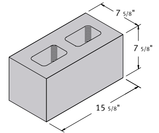
8 x 8 x 16 Semi Solid Pier
