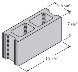
6 x 8 x 16 Hollow Stretcher
