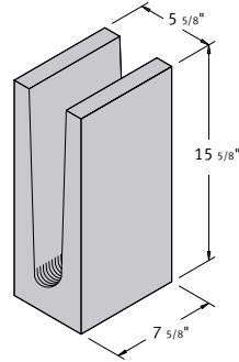
6 x 16 x 8 Bond Beam Lintel
