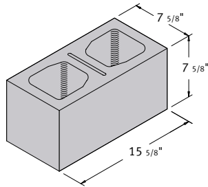
8 x 8 x 16 Hollow Pier
