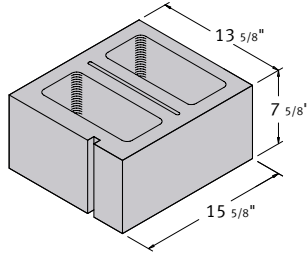
14 x 8 x 16 Hollow Corner Sash
