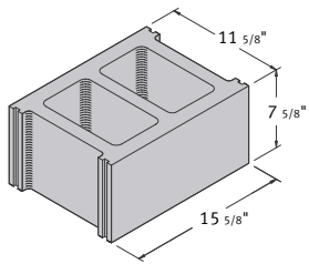
12 x 8 x 16 Hollow Stretcher
