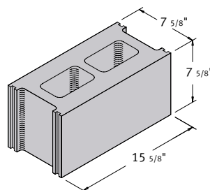
8 x 8 x 16 Hollow 3 Hour Fire Rated
