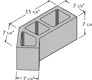
8 x 8 x 21 45 Degree Angle
