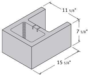
12 x 8 x 16 A Shaped Block
