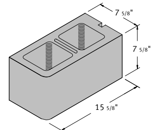
8 x 8 x 16 Hollow Single Bullnose Corner Sash
