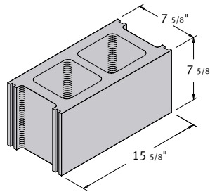
8 x 8 x 16 Hollow Stretcher
