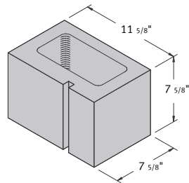
12 x 8 x 8 Hollow Corner Sash
