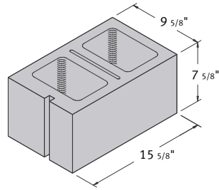
10 x 8 x 16 Hollow Corner Sash
