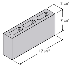
4 x 8 x 18 Hollow Pier
