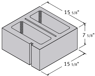
16 x 8 x 16 Hollow Corner Sash
