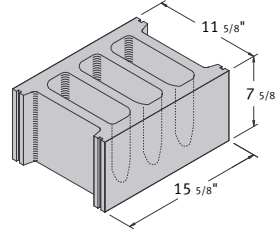
12 x 8 x 16 Hollow Cap 3 Core
