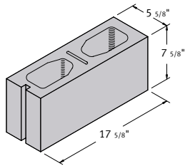
6 x 8 x 18 Hollow Corner Sash
