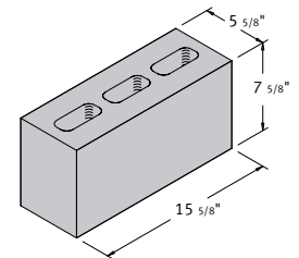
6 x 8 x 16 Semi Solid
