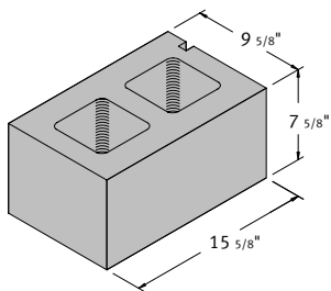
10 x 8 x 16 Semi Solid Corner Sash
