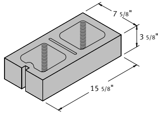
8 x 4 x 16 Hollow Corner Sash
