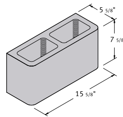
6 x 8 x 16 Hollow Single Bullnose Pier
