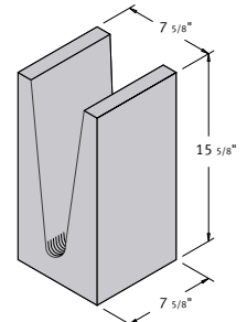
8 x 16 x 8 Bond Beam Lintel
