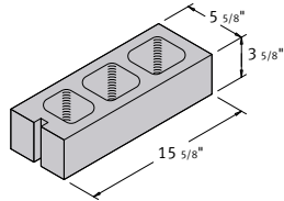
6 x 4 x 16 Hollow Corner Sash
