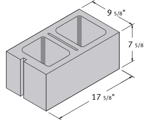
10 x 8 x 18 Hollow Corner Sash
