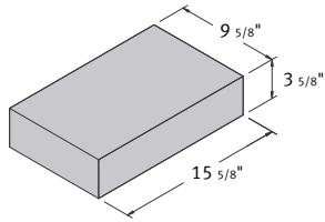
10 x 4 x 16 Solid Pier
