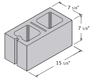
8 x 8 x 16 Hollow Corner Sash
