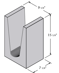
10 x 16 x 8 Bond Beam Lintel
