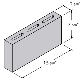
3 x 8 x 16 Hollow Pier
