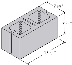
8 x 8 x 16 Hollow Double Sash
