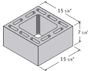
16 x 8 x 16 Chimney Block
