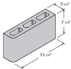
4 x 8 x 16 Hollow Single Bullnose Corner
