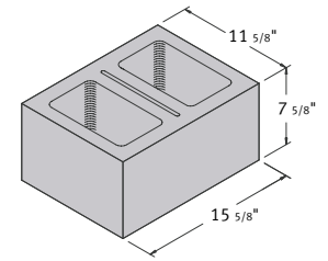
12 x 8 x 16 Hollow Pier
