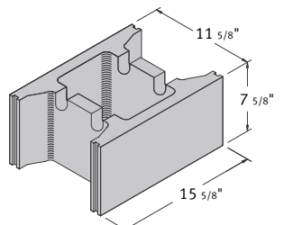
12 x 8 x 16 Open End
