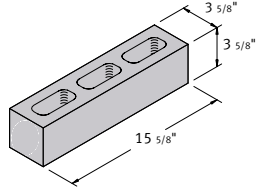
4 x 4 x 16 Hollow Pier
