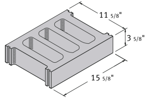
12 x 4 x 16 Hollow Stretcher
