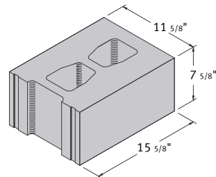
12 x 8 x 16 Semi Solid Single Corner Ear
