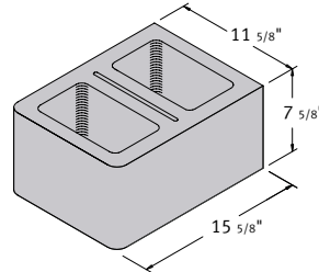
12 x 8 x 16 Hollow Double Bullnose Corner
