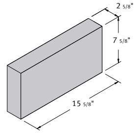
3 x 8 x 16 Solid Pier
