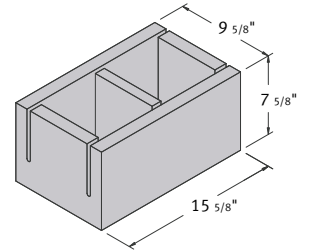
10 x 8 x 16 Knock-Out Bond Beam
