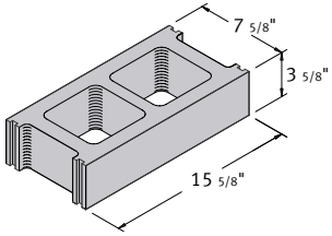
8 x 4 x 16 Hollow Stretcher
