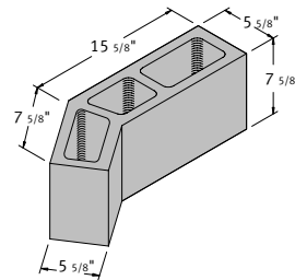
6 x 8 x 21 45 Degree Angle
