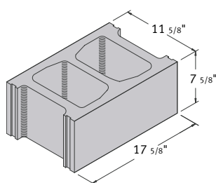
12 x 8 x 18 Hollow Stretcher
