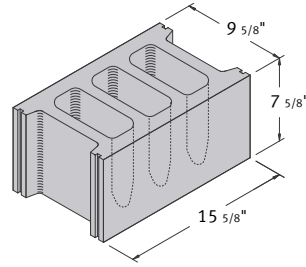
10 x 8 x 16 Hollow Cap 3 Core
