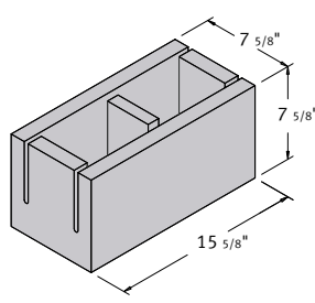
8 x 8 x 16 Knock-Out Bond Beam
